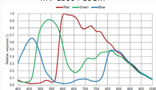
MV-CB004-10GC
