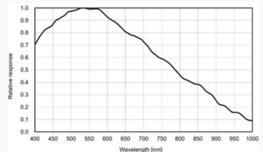
MV-CE200-11UM
