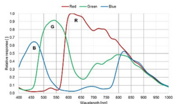
MV-CH120-10UC V4
