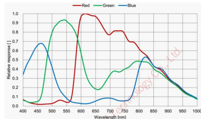
MV-CH310-10GC
