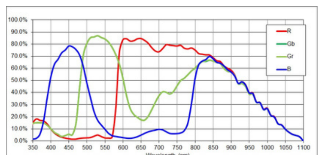
MV-CS050-60GC
