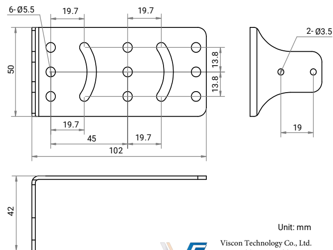
Installation Bracket:
